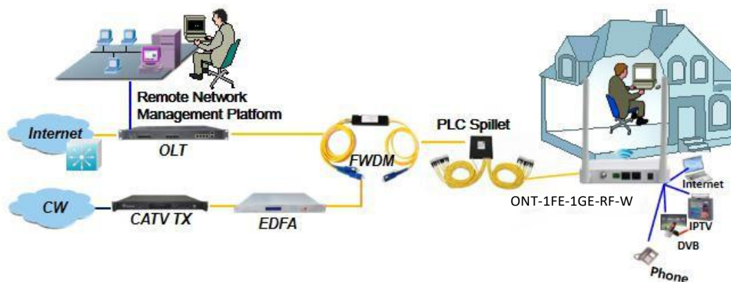
Figure: ONT-1FE-1GE-RF-W Application Diagram
